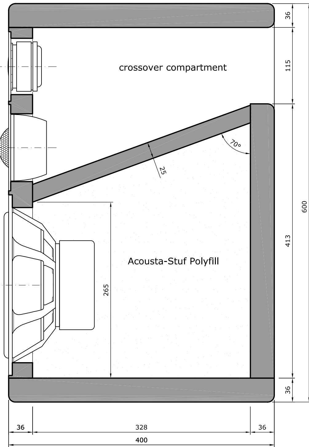
vertical section
