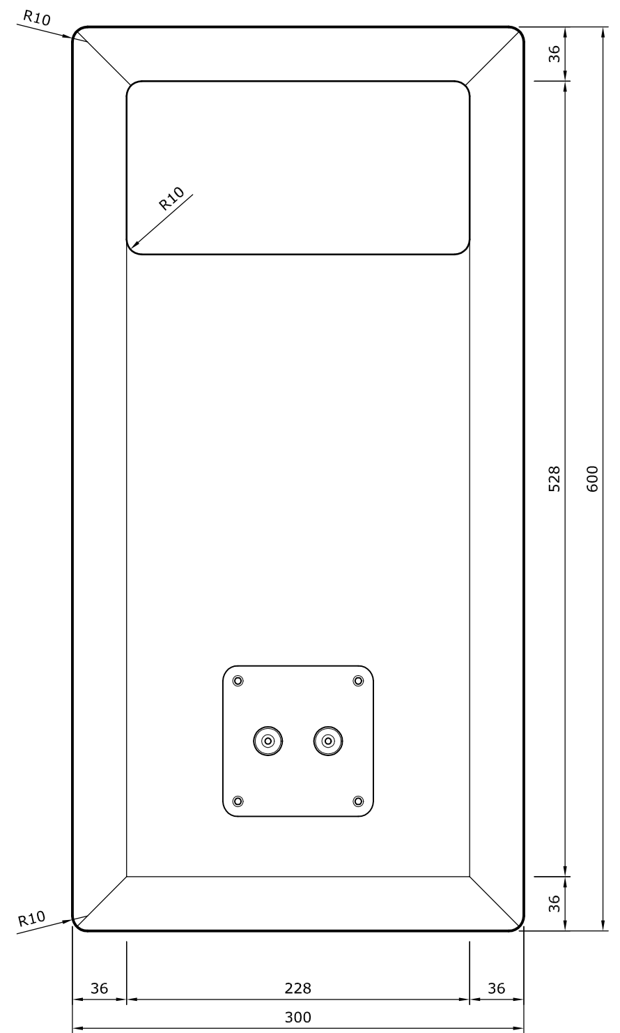
rear view
