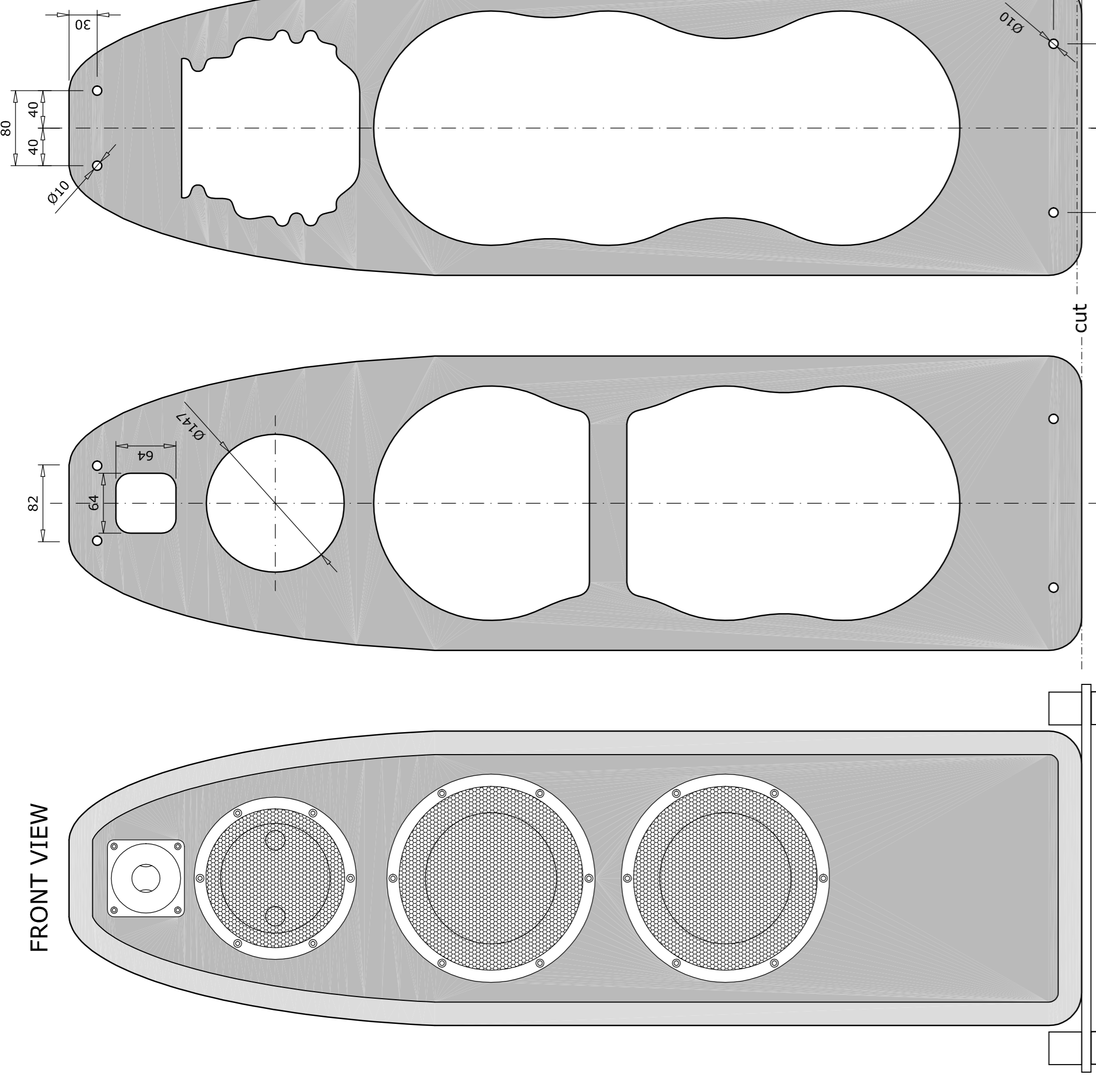
A - solidwood baffle 2x total
