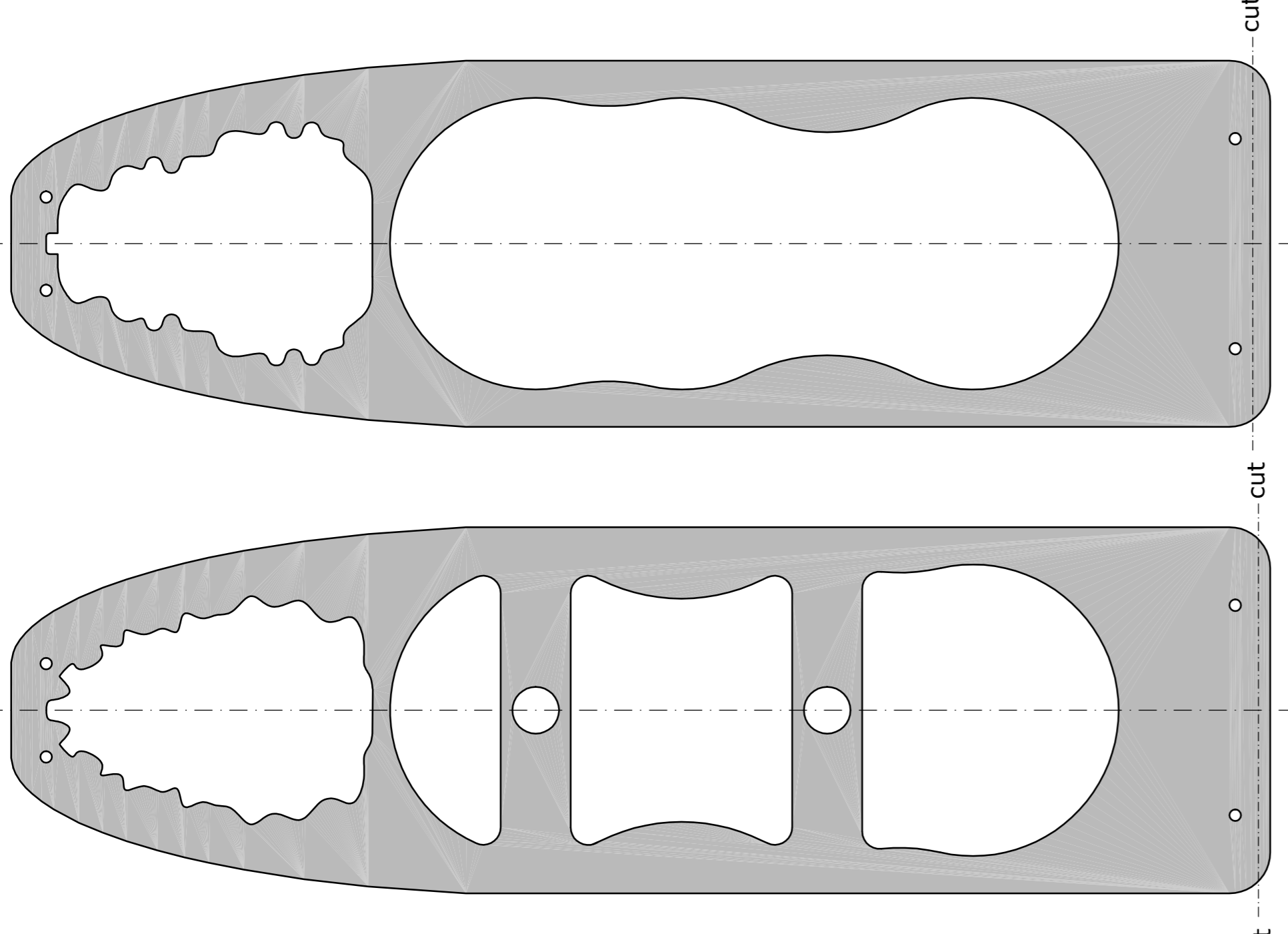
D - 38mm mdf panel 2x total
