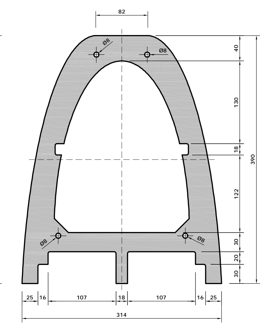
H - 16x vertical panel top-section
