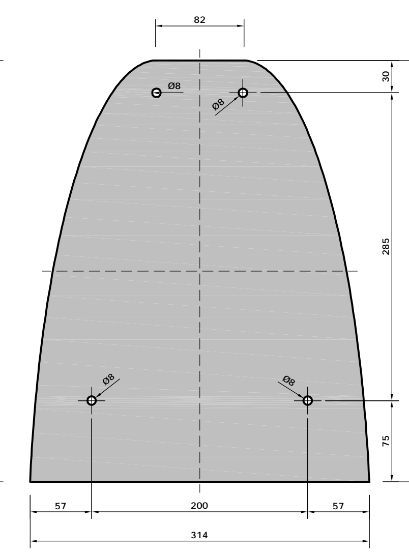
G - 8x vertical panel top-section
