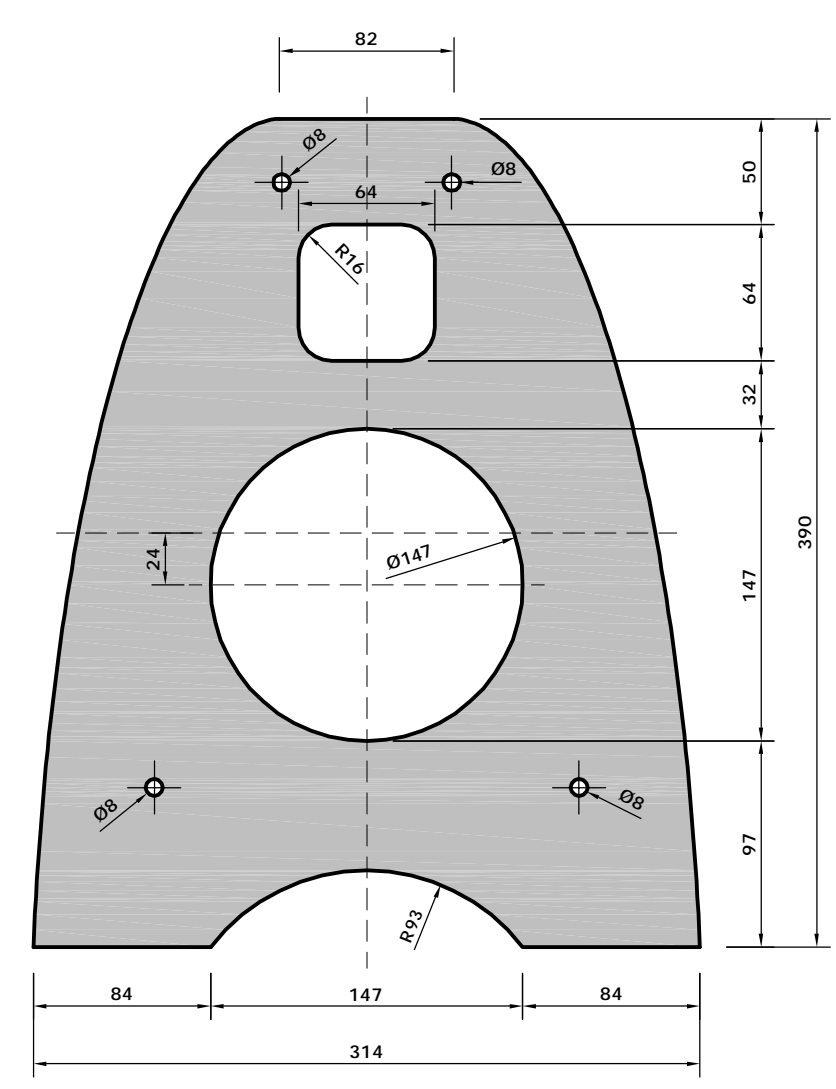
C - 2x vertical panel top-section
