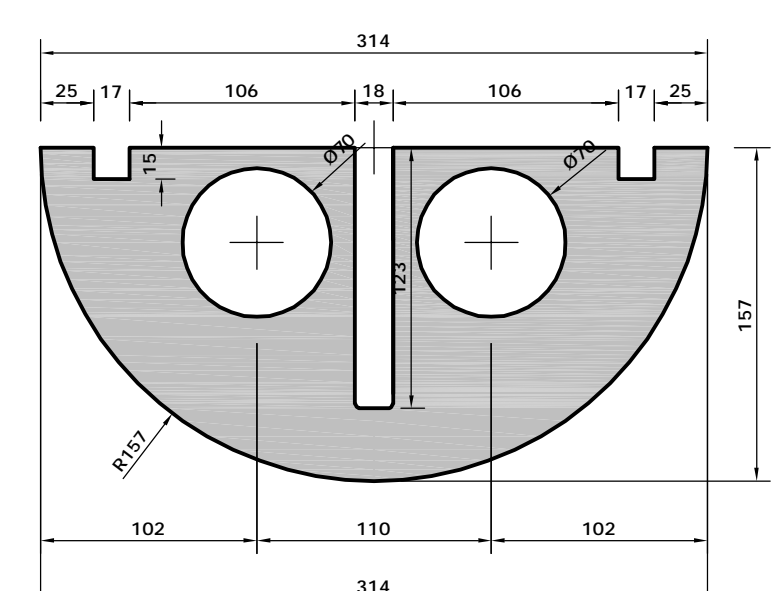
A - 8x horizontal panel bass-section
