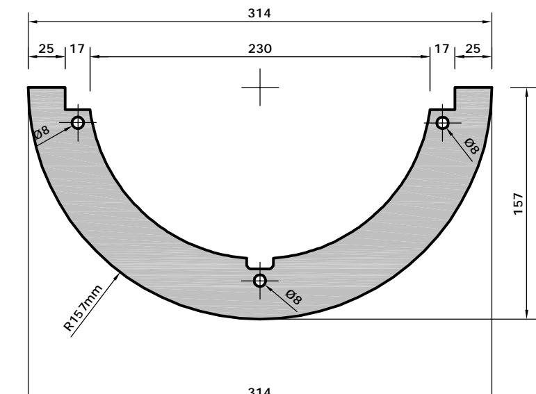
B - 50x horizontal panel bass-section
