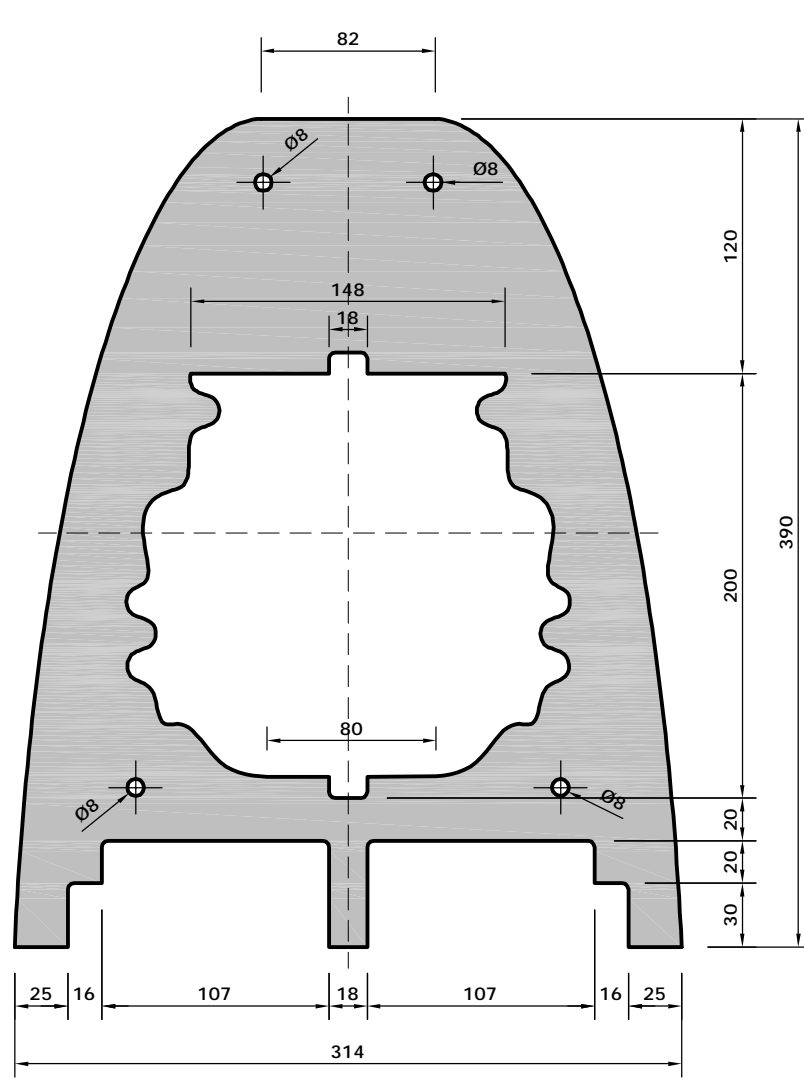
D - 2x vertical panel top-section
