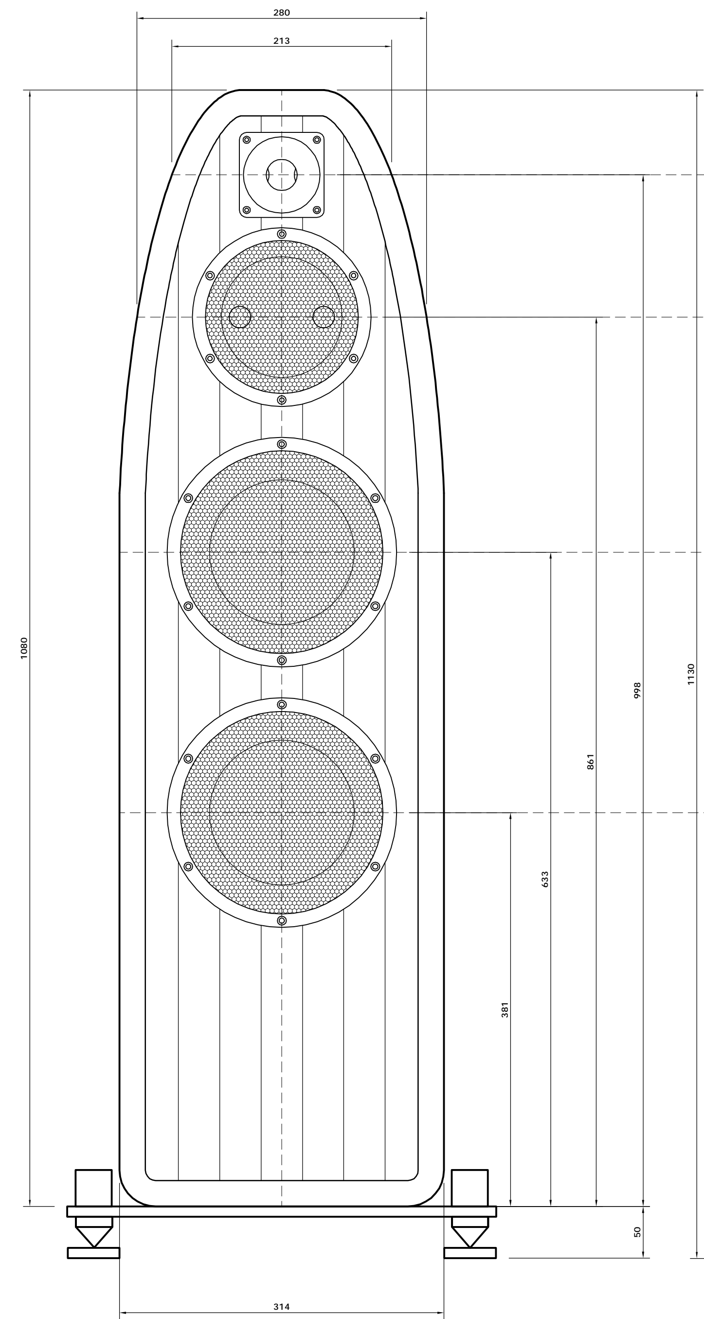
front view
