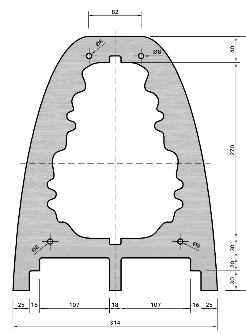
F - 6x vertical panel top-section
