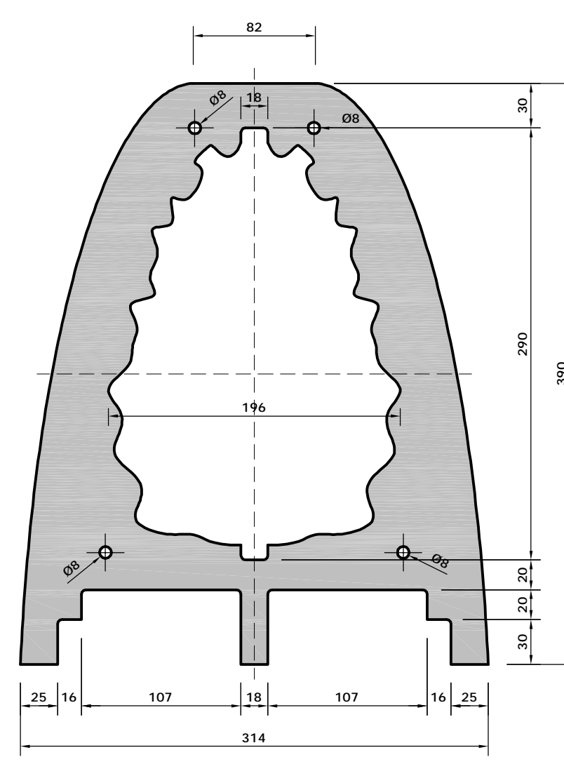
E - 6x vertical panel top-section
