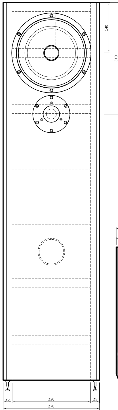
front view
