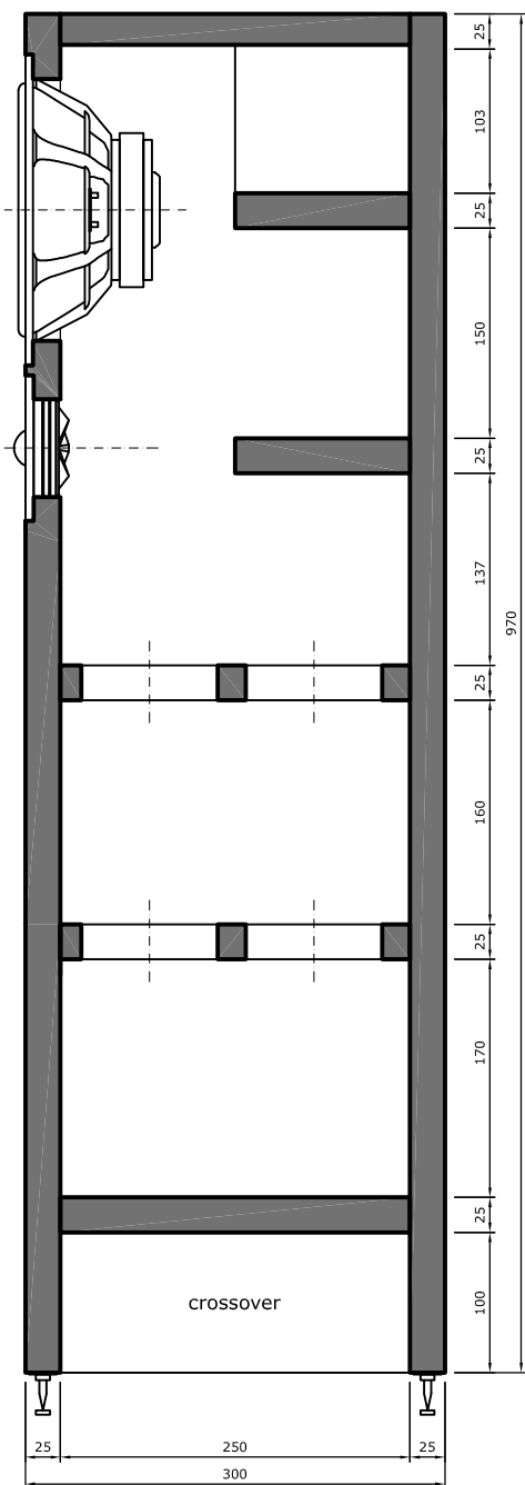
vertical section
