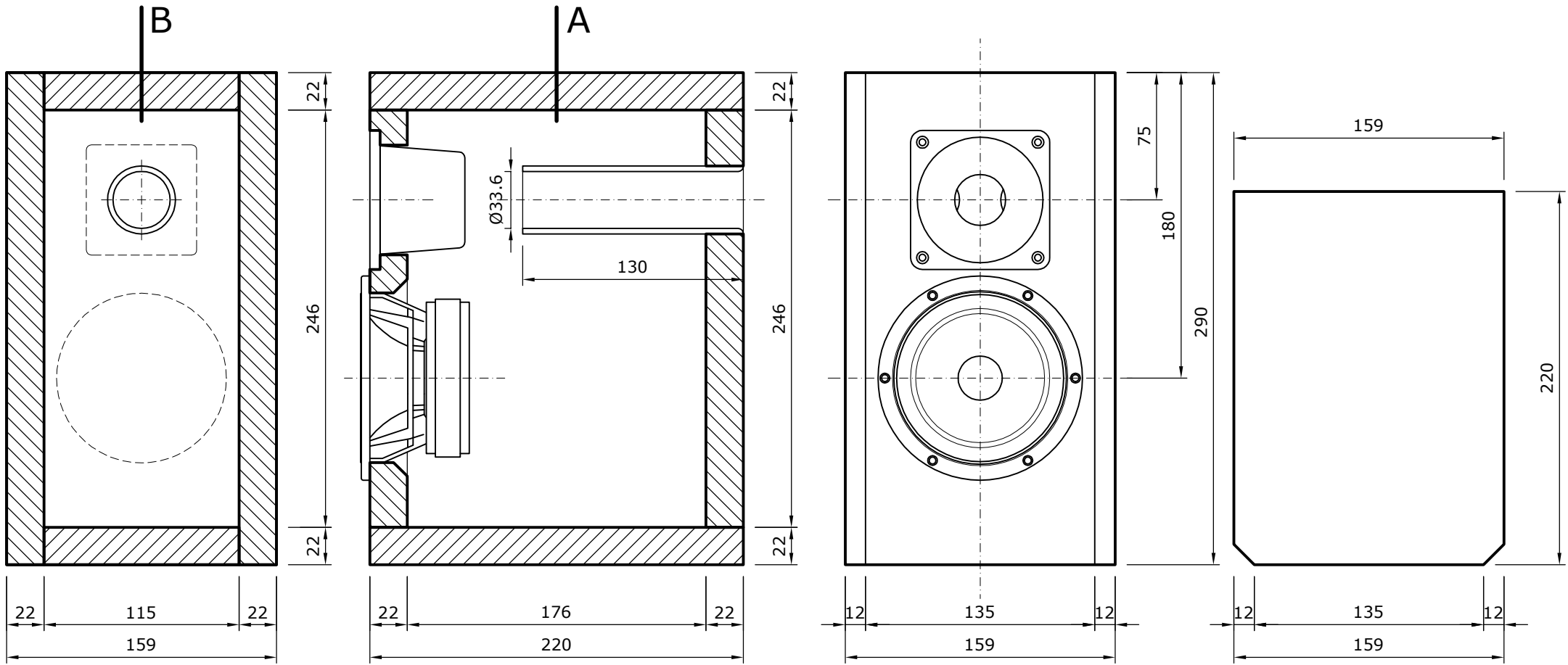
section A
