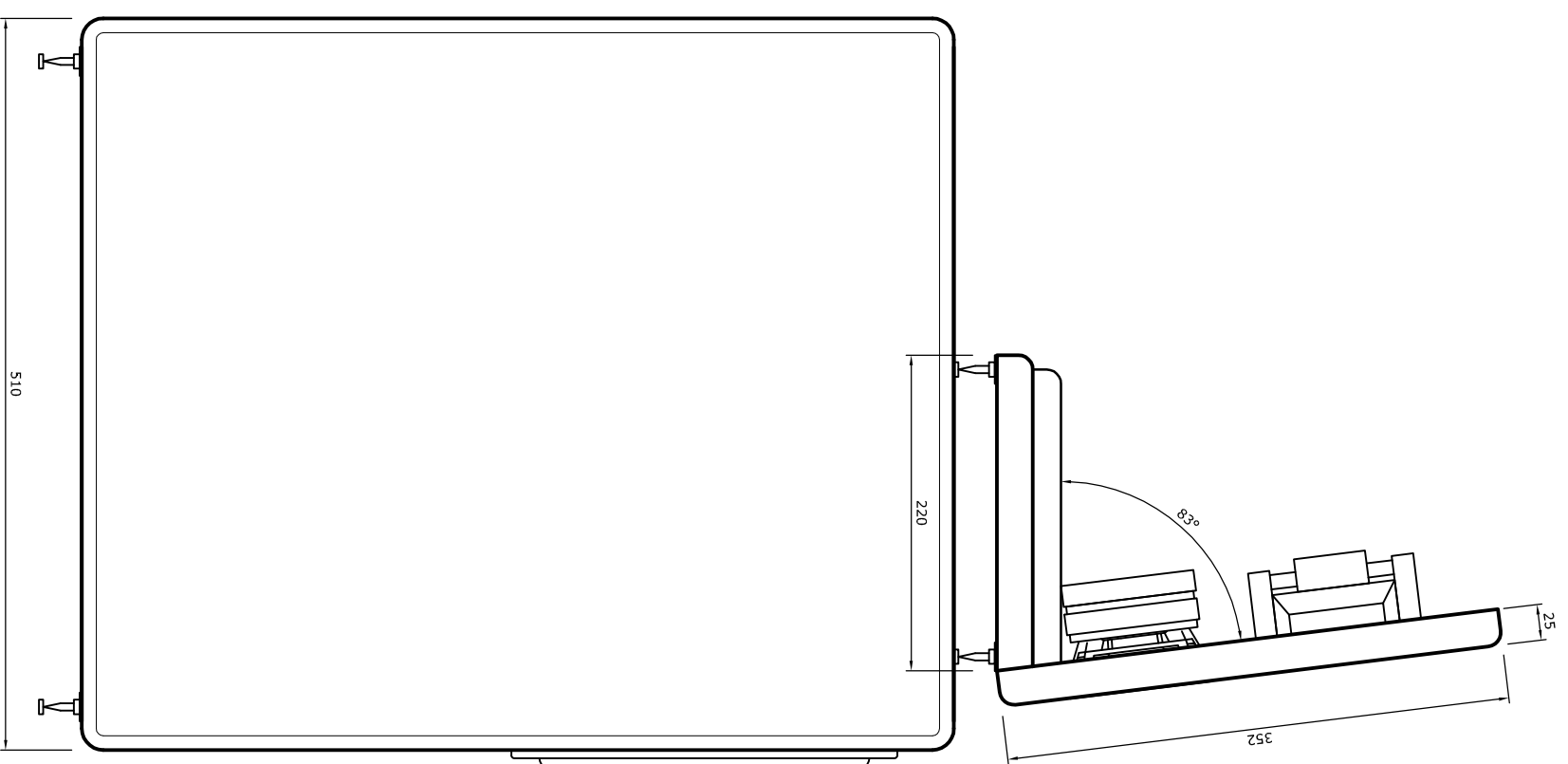
side view
