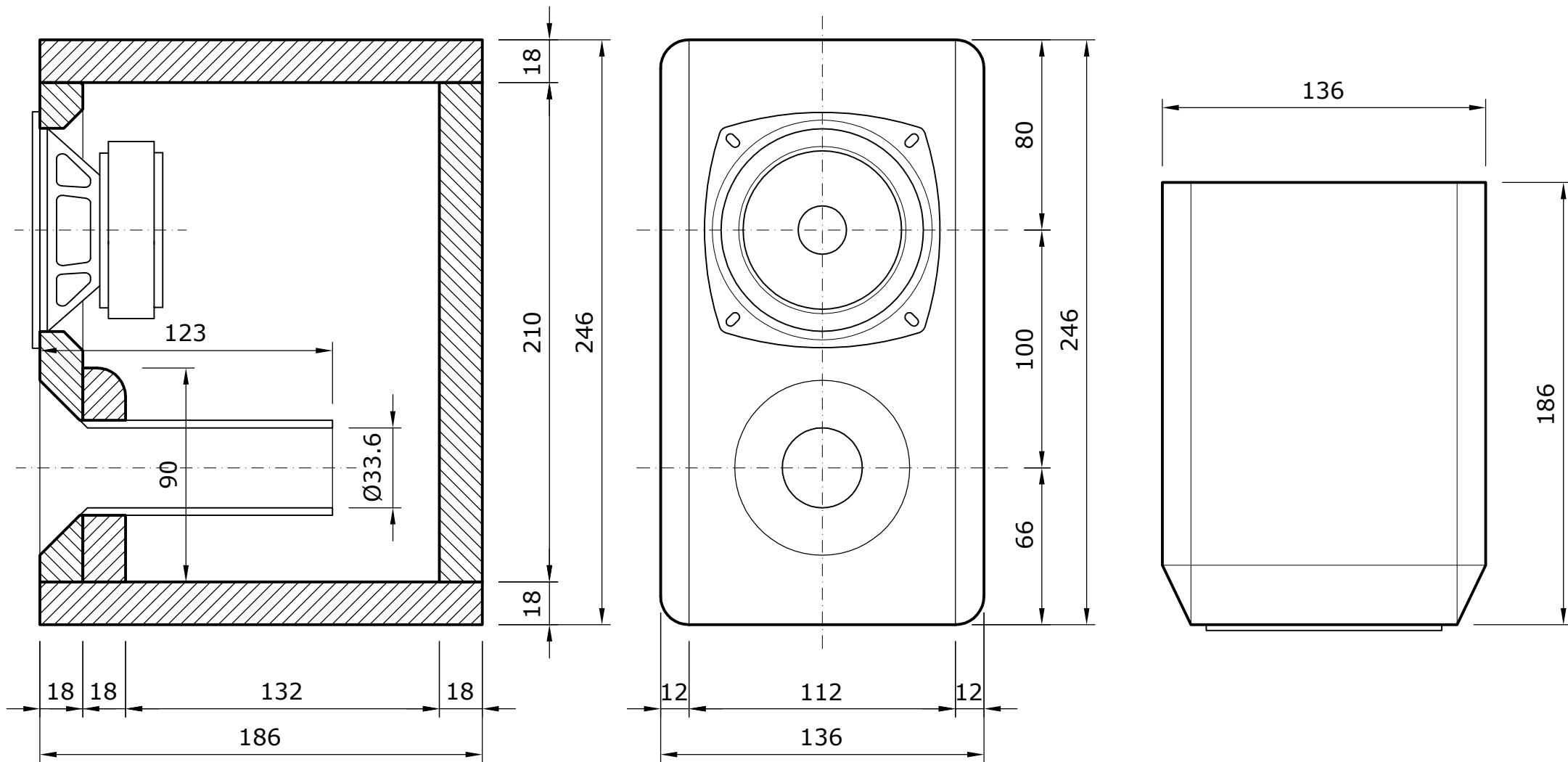
vertical section
