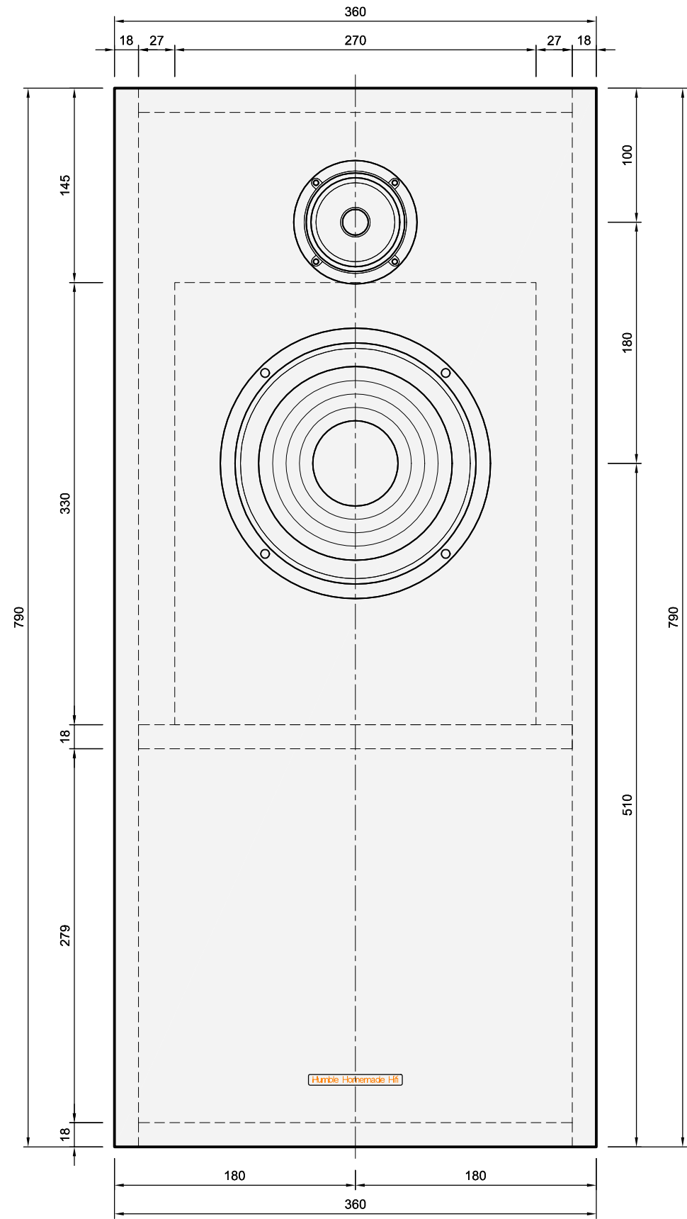
front view
