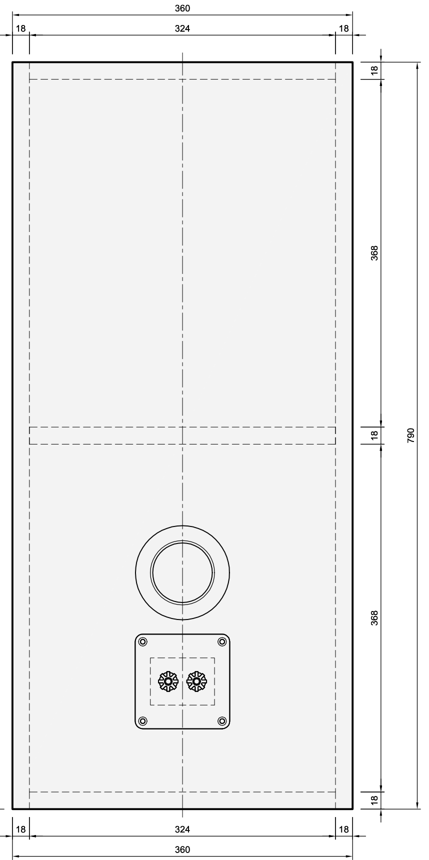
rear view
