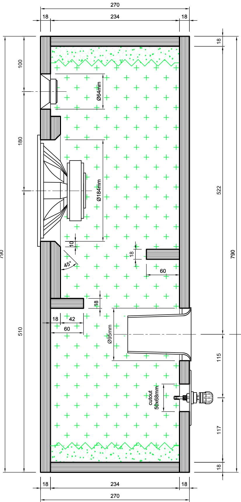
vertical section
